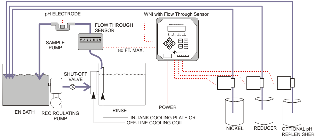
WNI with Flow Through Sensor, pH Electrode and Recirculating Pump
